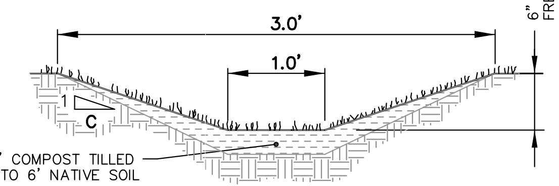
SECTION A-A (CONVEYANCE SWALE) NOT TO SCALE
