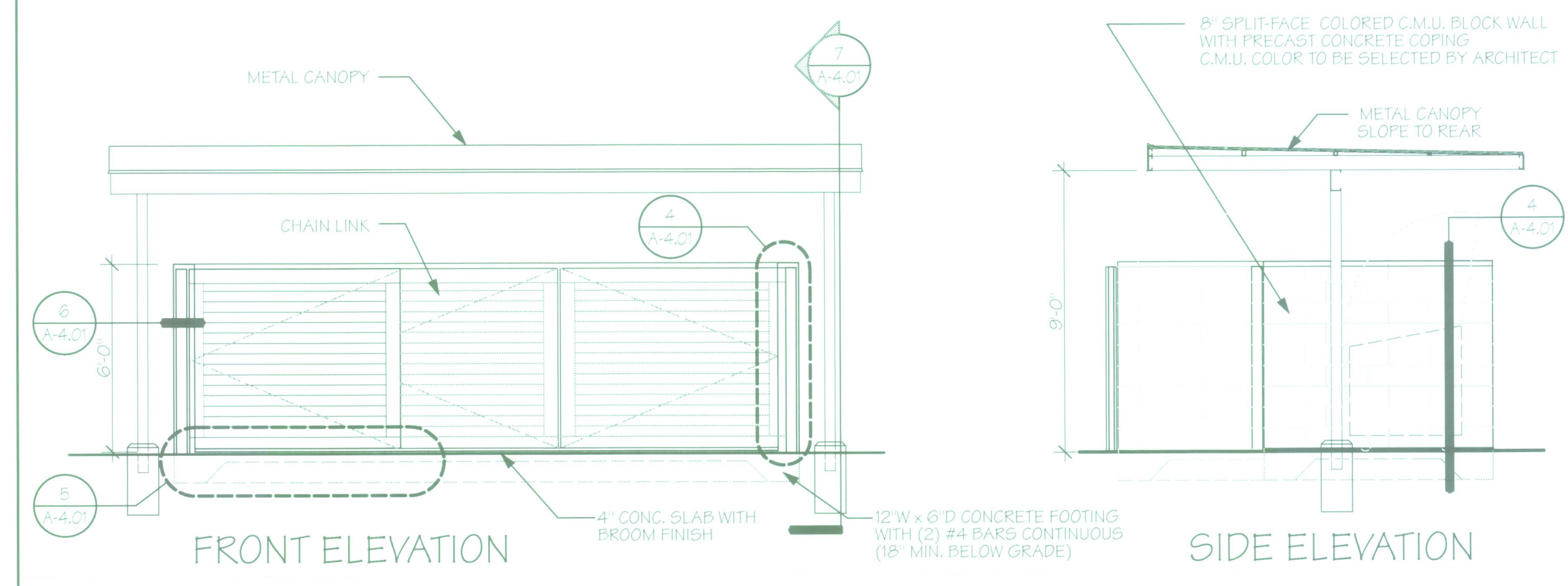
3 TRASH ENCLOSURE ELEVATIONS SCALE: 1/4" = 1'-0"
