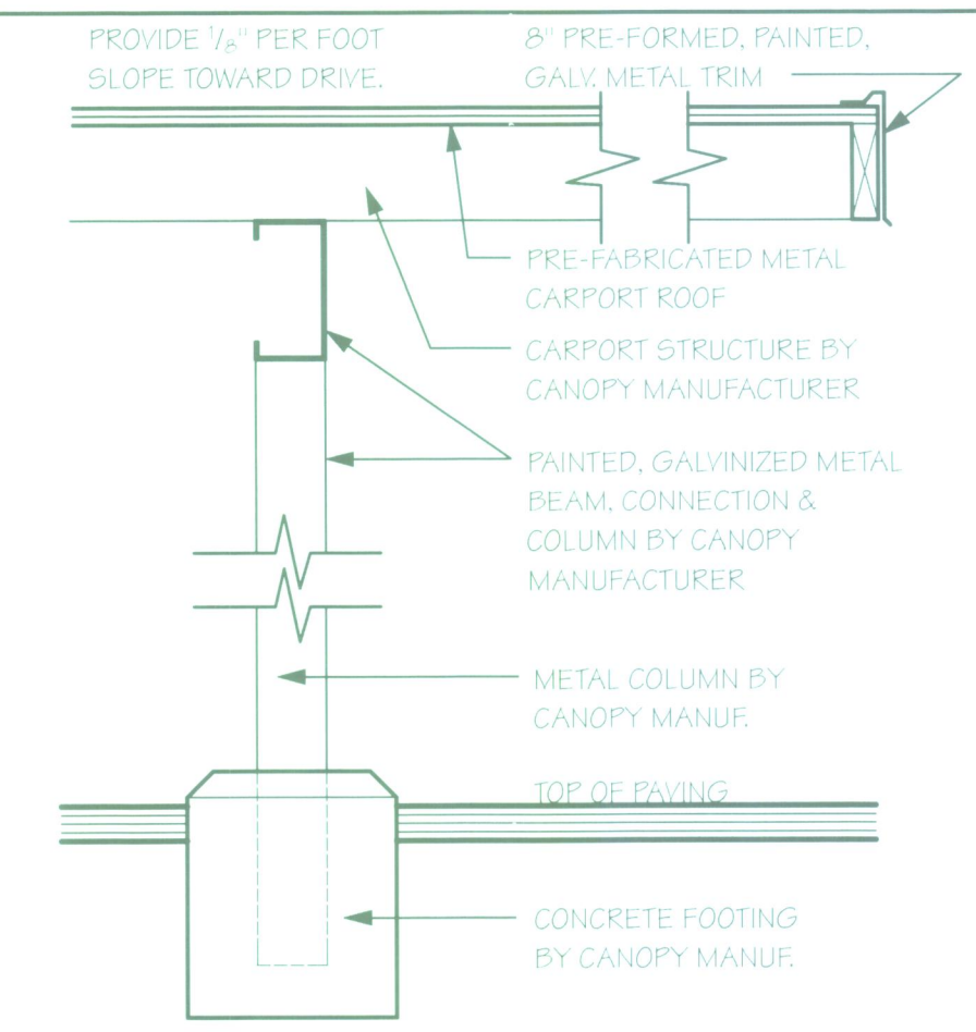
7 DUMPSTER CANOPY SECTION SCALE: 1" = 1'-0"
