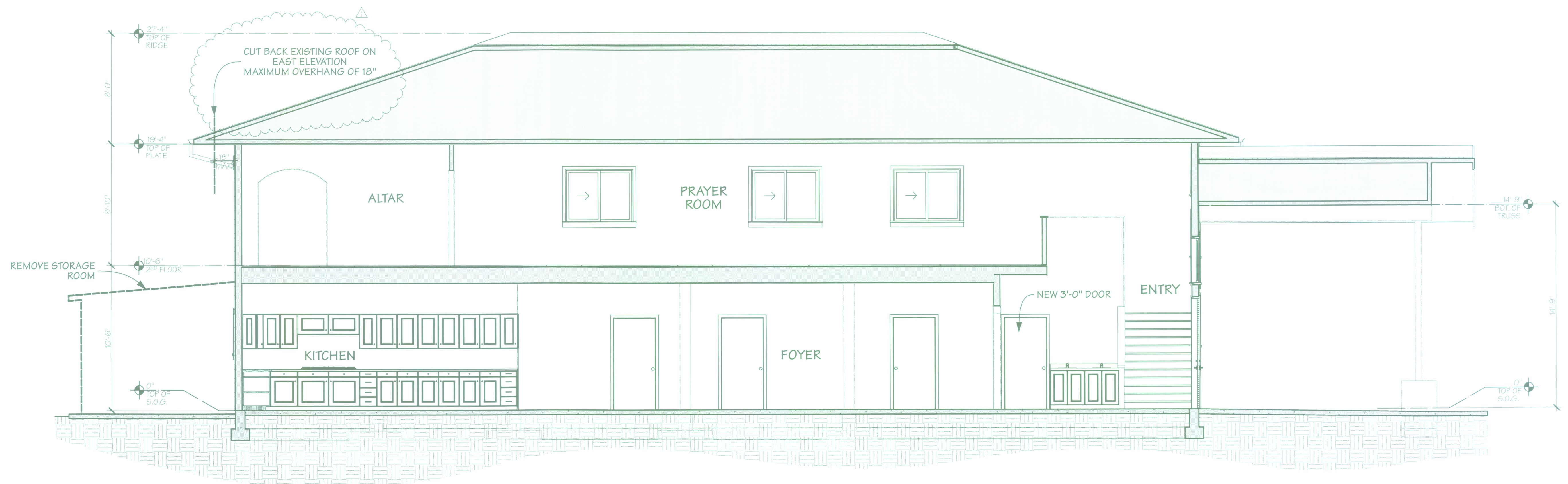
F SECTION F-F SCALE: 1/4" = 1'-0" 0 2 4 8
