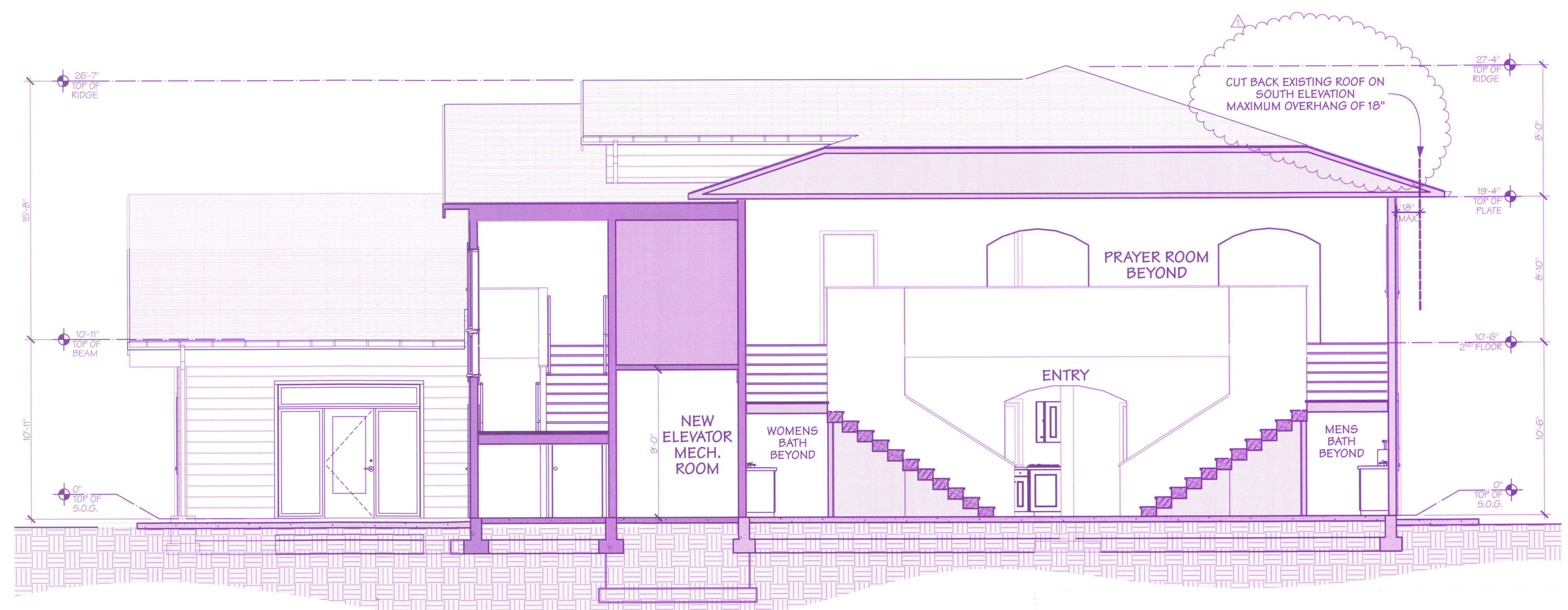
C SECTION C-C SCALE: 1/4" = 1'-0" 0 2' 4' 8'
