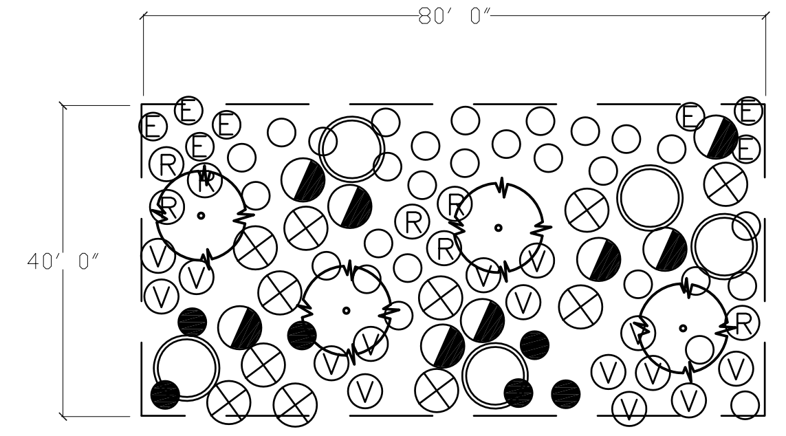
TYPICAL SHRUB LAYOUT— STEEP SLOPE/ PERIMETER BUFFER
