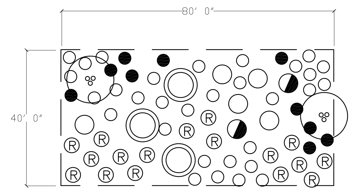
TYPICAL SHRUB LAYOUT— WETLAND/ STREAM BUFFER
